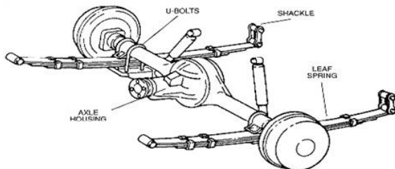
Figure 1: Suspension System of automobile
