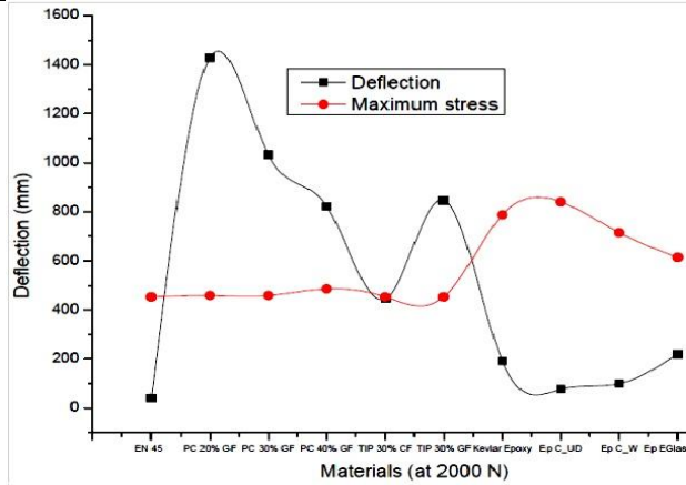
Figure 6: Deflection (mm) and maximum stress (MPa) at 2000 N
