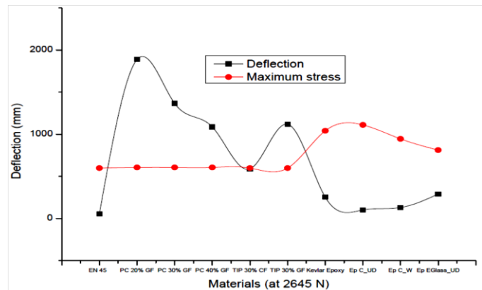
Figure 7: Deflection (mm) and maximum stress (MPa) at 2645 N
