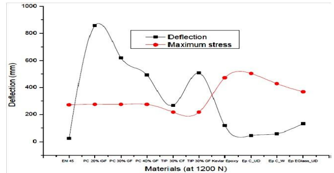
Figure 5: Deflection (mm) and maximum stress (MPa) at 1200 N
