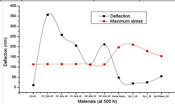
Figure 4: Deflection (mm) and maximum stress (MPa) at 500 N
