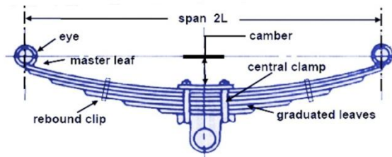
Figure 3: Leaf Spring
