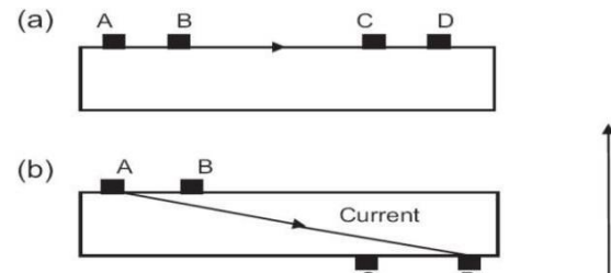
Figure 4. Different methods of electrical resistance measurement in self-sensing laminates.
