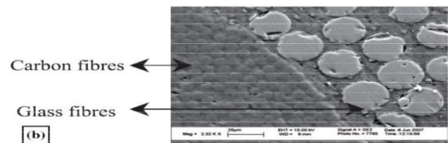
Figure 10. Structure of CF-GF hybrid composite rods for self-sensing: (a) schematic diagram (b) morphology.
