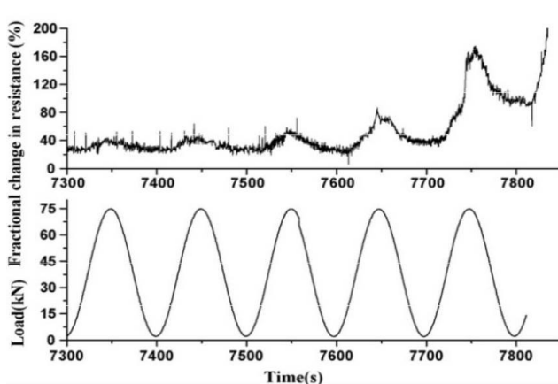
Figure 8. Fractional change in resistance during cyclic flexural loading at last 5 cycles.
