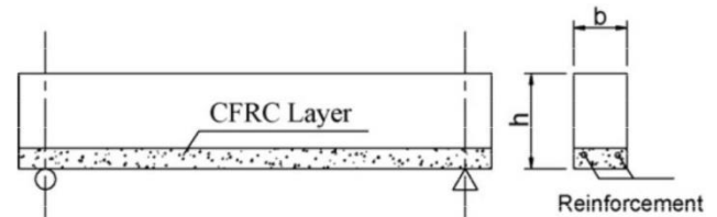
Figure 6. Schematic diagram of CFRC strengthened RC elements.
