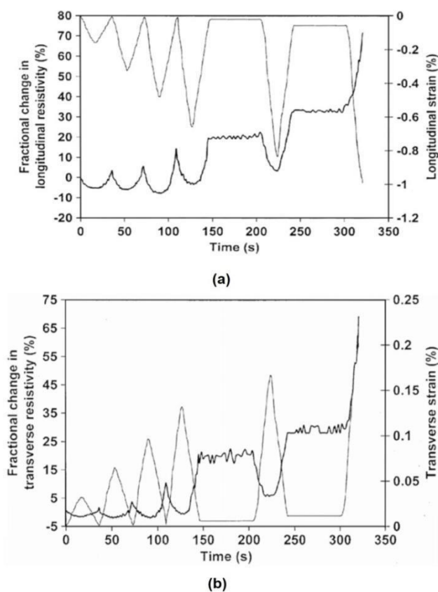
Figure 5. Variation of the fractional change in resistivity (thick curve) with time and strain (thin curve) with time during uniaxial compression at progressively increasing stress amplitudes: (a) longitudinal resistivity and (b) transverse resistivity that bridged the micro-cracks. The major damage was sensed by the irreversible increase in the specimen resistivity in the range of 10 to 30%. On the contrary, smaller change in resistivity ranging from 1 to
