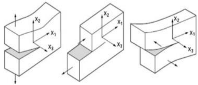
Figure 1: Three types of loading on a cracked body
