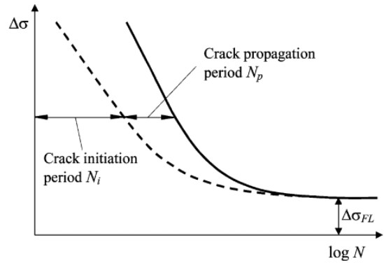
Figure 3: Schematic representation of the service life of mechanical elements.
