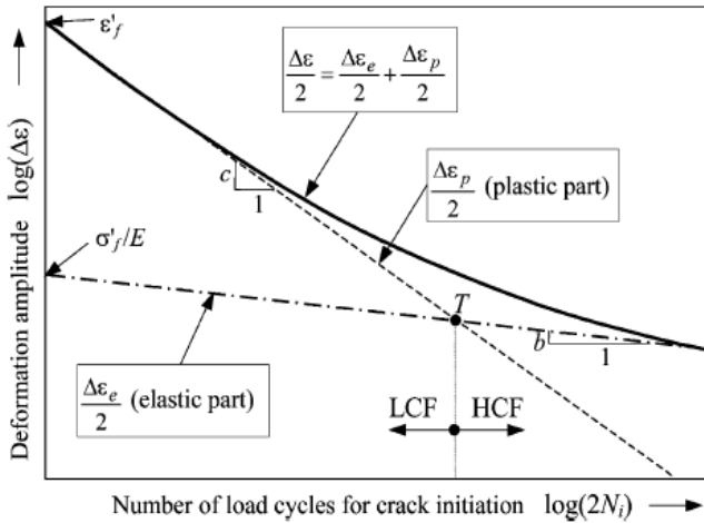
Figure 5: Strain-life ( \epsilon - N_i ) method for the fatigue crack initiation
