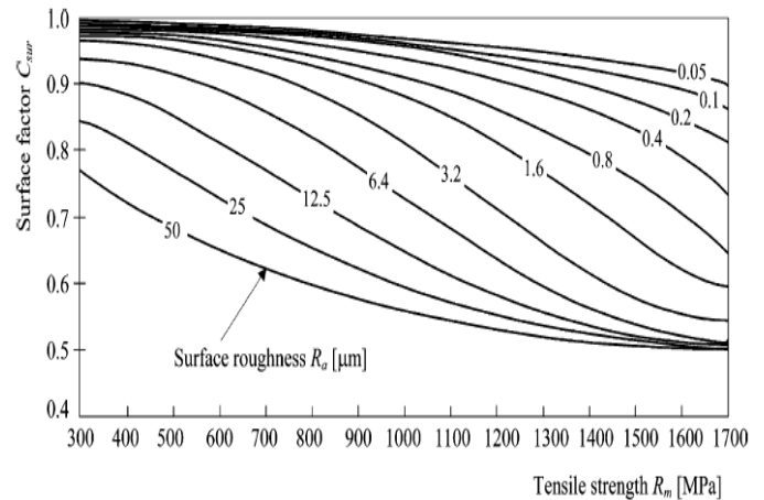
Figure 6: Surface finish correction factor
