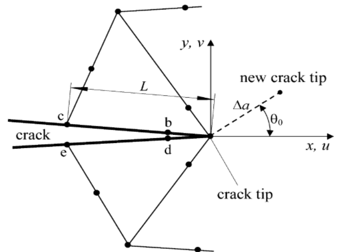
Figure 7: Triangular quarter-point elements around crack tip
